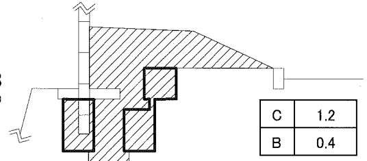
No. 4+5.8 (B-B' 断面部)
