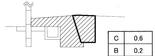
No. 6+6.0 (D-D' 断面部)
