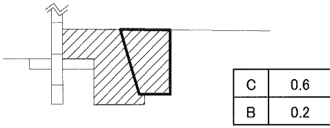
No. 5+2.8' (D-D' 断面部)
