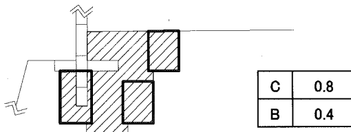
No. 4+16.5 (C-C' 断面部)
